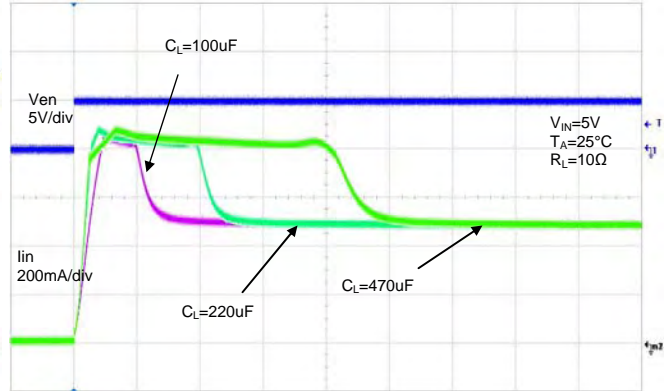
Inrush Current
